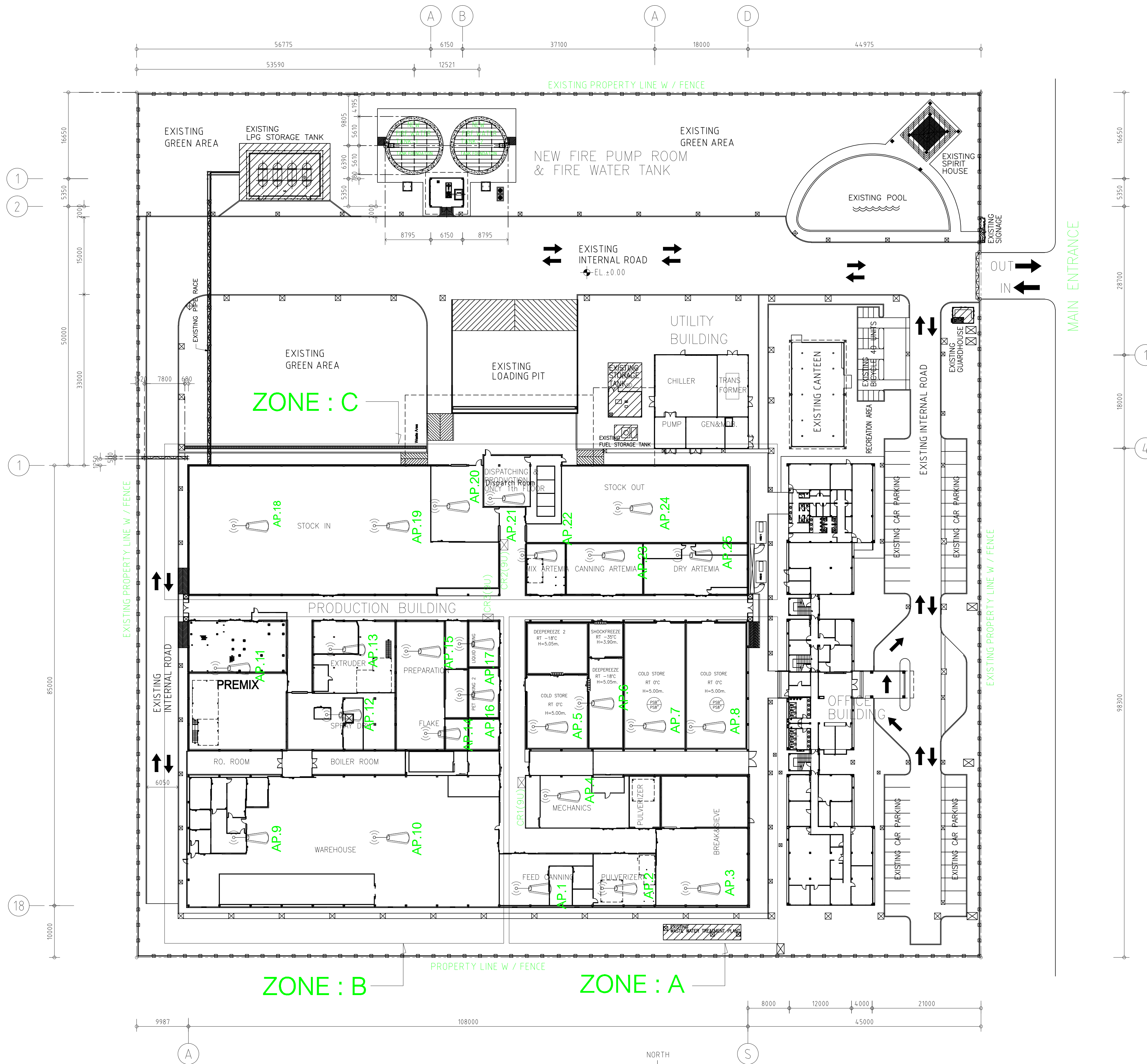
SITE LAYOUT SCALE 1:400
